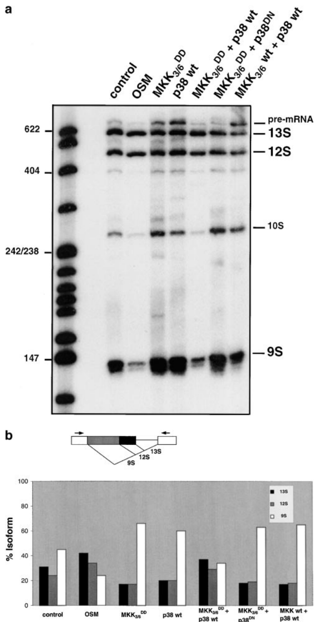
Figure 7. Activation of the MKK 3/6 -p38 pathway and the concomitant reduction of the level of nuclear hnRNP A1 correlates with changes in alternative splicing. COS cells were transiently transfected with 6 \mu g of plasmid encoding the E1A splicing reporter minigene alone or together with 7 \mu g of expression plasmids encoding myc-tagged versions of the MKK 3/6 kinase, or its permanently active mutant (MKK 3/6 DD ), in conjunction with 7 \mu g of expression plasmids encoding HA-tagged versions of wild-type p38 kinase or its dominant-negative mutant (p38 DN ). At 24 h after transfection cells were either left untreated or exposed to 600 mM sorbitol for 4 h. Total RNA was then isolated and the alternative splicing pattern of the E1A transcripts was determined by RT-PCR. The relative levels of 13S, 12S, and 9S mRNAs were quantitated as described (Cáceres et al., 1994; Sreaton et al., 1995). The E1A transcript isoforms are shown schematically. Essentially identical results were obtained in three independent experiments.
