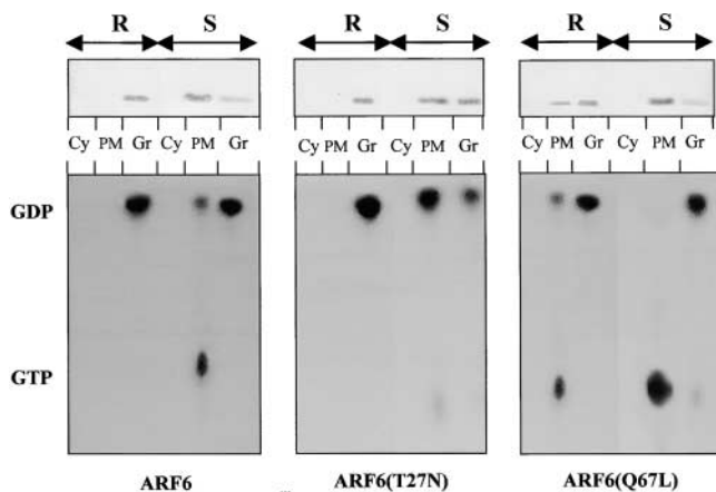
Figure 5. Nucleotide status of ARF6 in resting and stimulated PC12 cells. PC12 cells expressing HA-ARF6 or HA-ARF6 mutants were labeled with [ ^{32} P]orthophosphate and then incubated in Locke (R) or 59 mM K^+ (S) for 15 min. Cells were processed for subcellular fractionation and HA-tagged ARF6 proteins were immunoprecipitated from the cytosol (Cy), plasma membrane (PM), and secretory granules (Gr). (Top) 5 \mu l aliquots were analyzed by electrophoresis and Western blotting using anti-ARF6 antibodies. (Bottom) Guanine nucleotides eluted from the HA-immunoprecipitated ARF6 proteins were separated on chromatography plates and subjected to autoradiography. Similar results were obtained from three different cell preparations.
