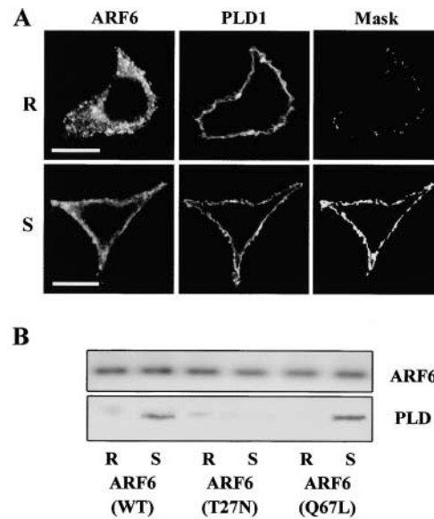
Figure 9. ARF6 interacts with PLD1 in stimulated PC12 cells. (A) PC12 cells cotransfected with pEGFP-PLD1 and pXS-ARF6 were incubated for 5 min in either Locke's solution (R) or in 59 mM K^+ (S). Cells were subsequently stained with rabbit anti-ARF6 antibodies. Masks representing the regions of colocalization were generated by selecting the double-labeled pixels. Bars, 10 \mu m. (B) PC12 cells expressing HA-ARF6 or HA-ARF6 mutants were incubated for 10 min in either Locke's solution (R) or in 59 mM K^+ (S). Cells were scrapped and HA-tagged ARF6 proteins were immunoprecipitated. Samples were analyzed by electrophoresis and Western blotting using anti-ARF6 and anti-PLD1 antibodies. Similar results were obtained from three different cell preparations.
