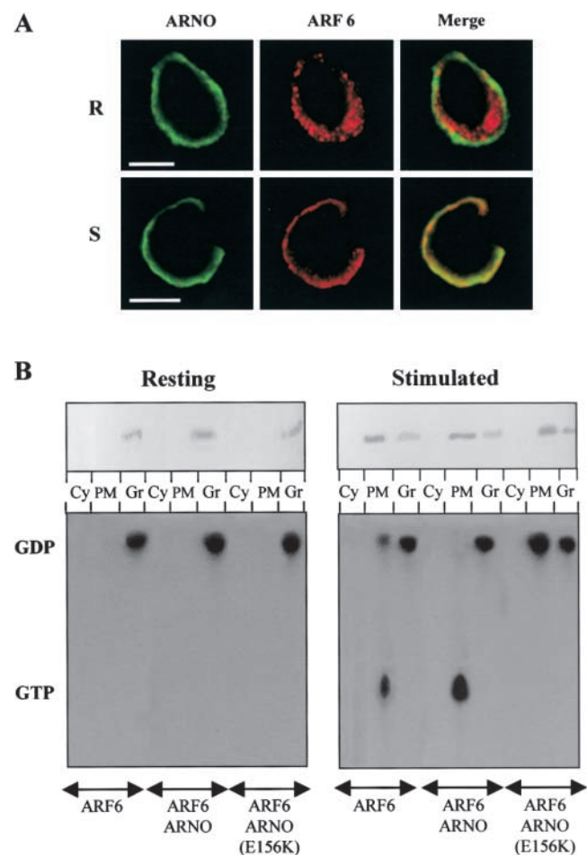
Figure 6. ARF6 is activated by ARNO at the plasma membrane in stimulated PC12 cells. (A) PC12 cells transfected with pXS-ARF6 in combination with the pCB7-myc-ARNO expression plasmid were incubated in Locke (R) or stimulated with 59 mM K^+ (S) for 5 min. After fixation, cells were stained with monoclonal anti-myc (ARNO) and rabbit polyclonal anti-ARF6 antibodies. In the merge images, the yellow-orange staining indicates the areas of colocalization between ARNO and ARF6. Bars, 5 \mu m. (B) PC12 cells transfected with pXS-ARF6 in combination with pCB7, pCB7-myc-ARNO, or pCB7-myc-ARNO(E156K) were labeled with [ ^{32} P]orthophosphate and then incubated in Locke (Resting) or stimulated with 59 mM K^+ (Stimulated). Cells were subsequently processed for subcellular fractionation and HA-ARF6 was immunoprecipitated from the cytosol (Cy), the plasma membrane (PM), and the secretory granules (Gr). (Top) 5 \mu l aliquots were analyzed by Western blotting using anti-ARF6 antibodies. (Bottom) guanine nucleotides bound to HA-ARF6 were analyzed by chromatography. Identical results were obtained with two independent cell preparations.
