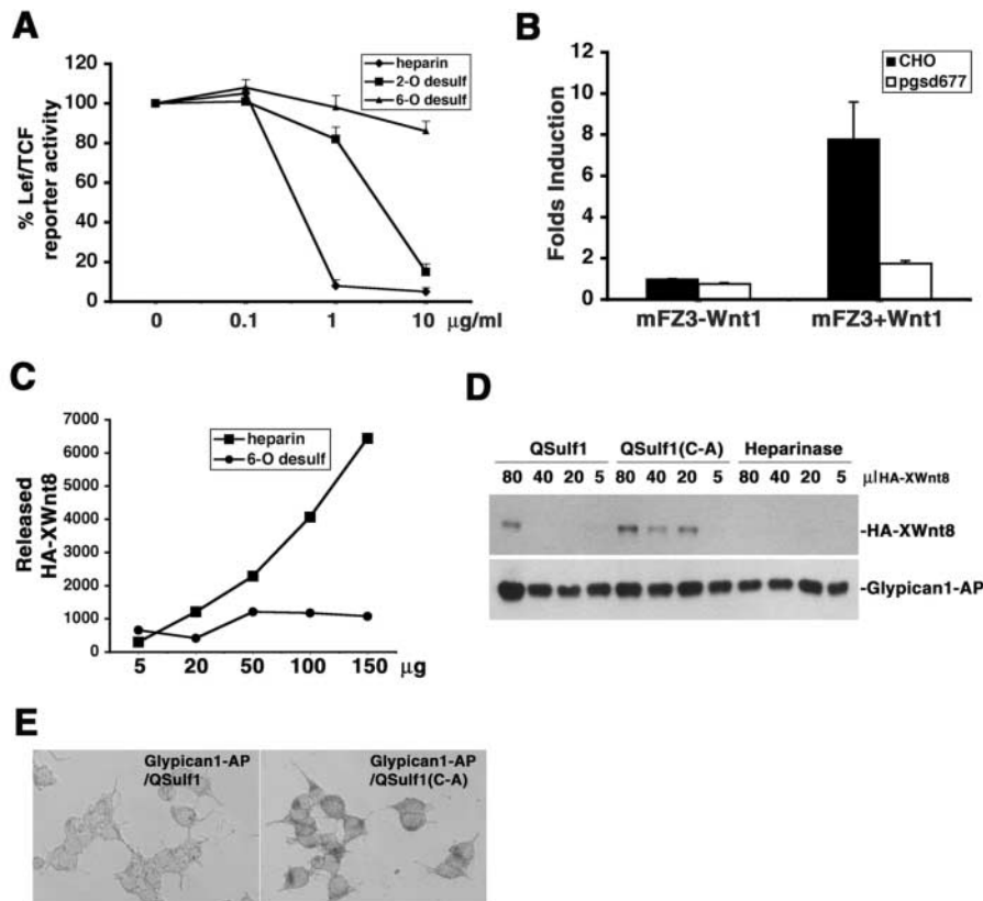
Figure 5. QSulf1 regulates the interaction between HS and Wnt ligand to promote Wnt signaling.
