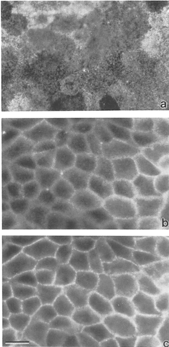
Figure 9. Localization of gp23 on the MDCK TX-100 cytoskeleton. Confluent cells were incubated in either CSK buffer (a) or CSK buffer containing 0.5% TX-100 (b and c) for 15 min at 4°C and gp23 distribution was determined by immunofluorescence microscopy. After CSK buffer treatment (a), intense staining of gp23 was demonstrated on the apical cell surface. On TX-100 cytoskeletons (b), gp23 staining was greatly reduced at the apical cell surface. However, when the same monolayer was viewed with the focal plane in the center of the cell (c), intense gp23 was observed on the basolateral membranes. Bar, 20 \mu m.
