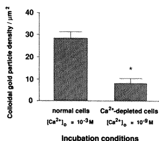
Figure 7. Density of colloidal gold particles per squared micron of phagosomal space (see Materials and Methods) in neutrophils incubated in \text{Ca}^{2+} medium or in MAPT/AM loaded neutrophils in \text{Ca}^{2+} -free medium. n = 80 , number of pictures of different phagosomal spaces analyzed from two different experiments. * P < 0.001 .
