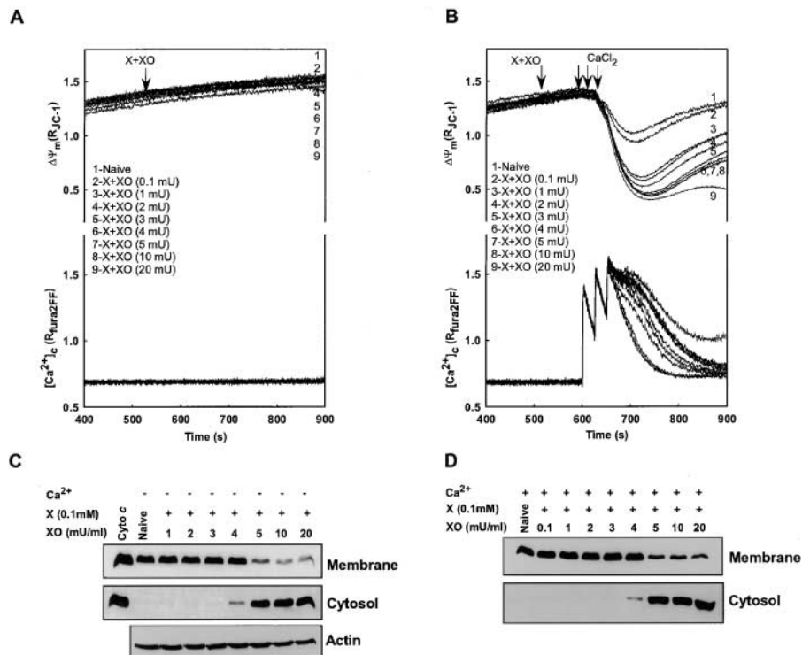
Figure 2. Ca 2+ -induced mitochondrial depolarization is not essential for O 2 ·- -dependent CCR. Permeabilized cells were treated with X (0.1 mM) and different concentrations of XO (0.1, 1, 2, 3, 4, 5, 10, or 20 mU/ml) before addition of Ca 2+ pulses (30 μM each) or solvent. (A and B) ΔΨ m measured simultaneously with [Ca 2+ ] c . (C and D) cyto c in the cytosol and membrane fractions. Immunoblotting of actin in the cytosolic fraction was used to evaluate whether O 2 ·- changed the distribution of nonmitochondrial proteins.
