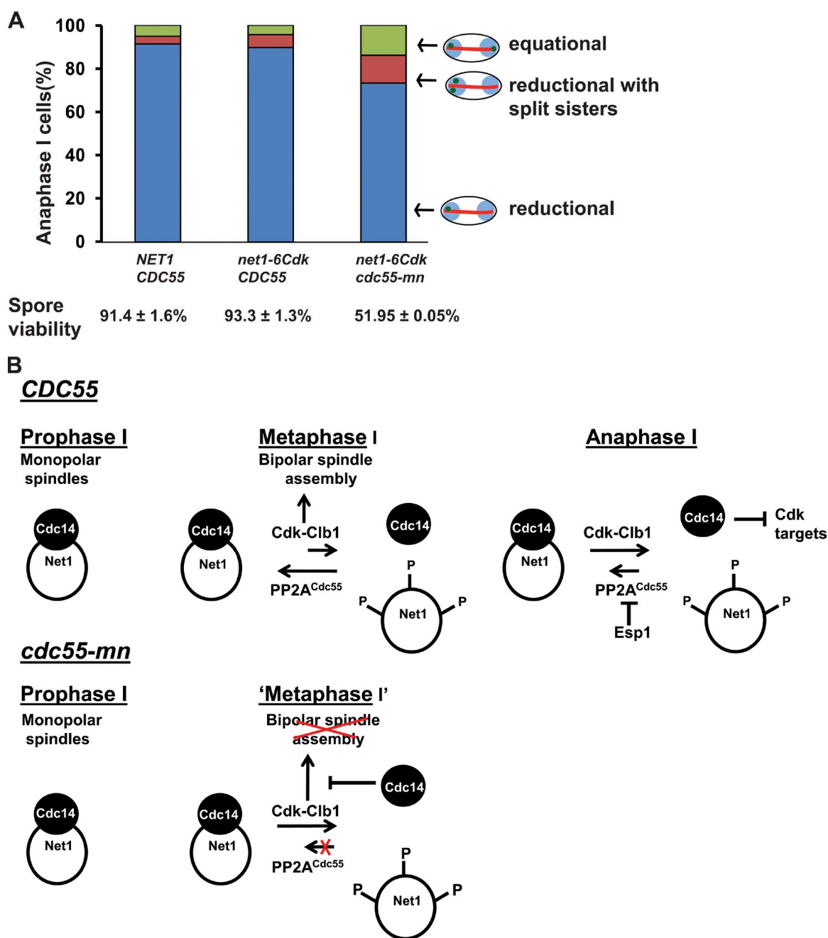
Figure 5. Analyses of spore viability and sister centromere segregation during meiosis I in net1-6Cdk cdc55-mn cells and a model for PP2A Cdc55 's role in preventing premature exit from meiosis I. (A) NET1 CDC55 , net1-6Cdk CDC55 , and net1-6Cdk cdc55-mn cells from the same experiment described in Fig. 4 A were stained against tubulin, and the segregation of GFP-tagged sister centromeres was examined in cells containing anaphase I spindles ( n = 100 ). Representative data from three experimental repeats are indicated. Spore viabilities of the aforementioned strains were obtained after dissecting 100 spores from tetrads onto YEPD plates followed by incubation at 25°C for 3 d. Values indicated represent means obtained from two independent experiments. (B) See the last paragraph of the Discussion for details. P, phosphorylation.
