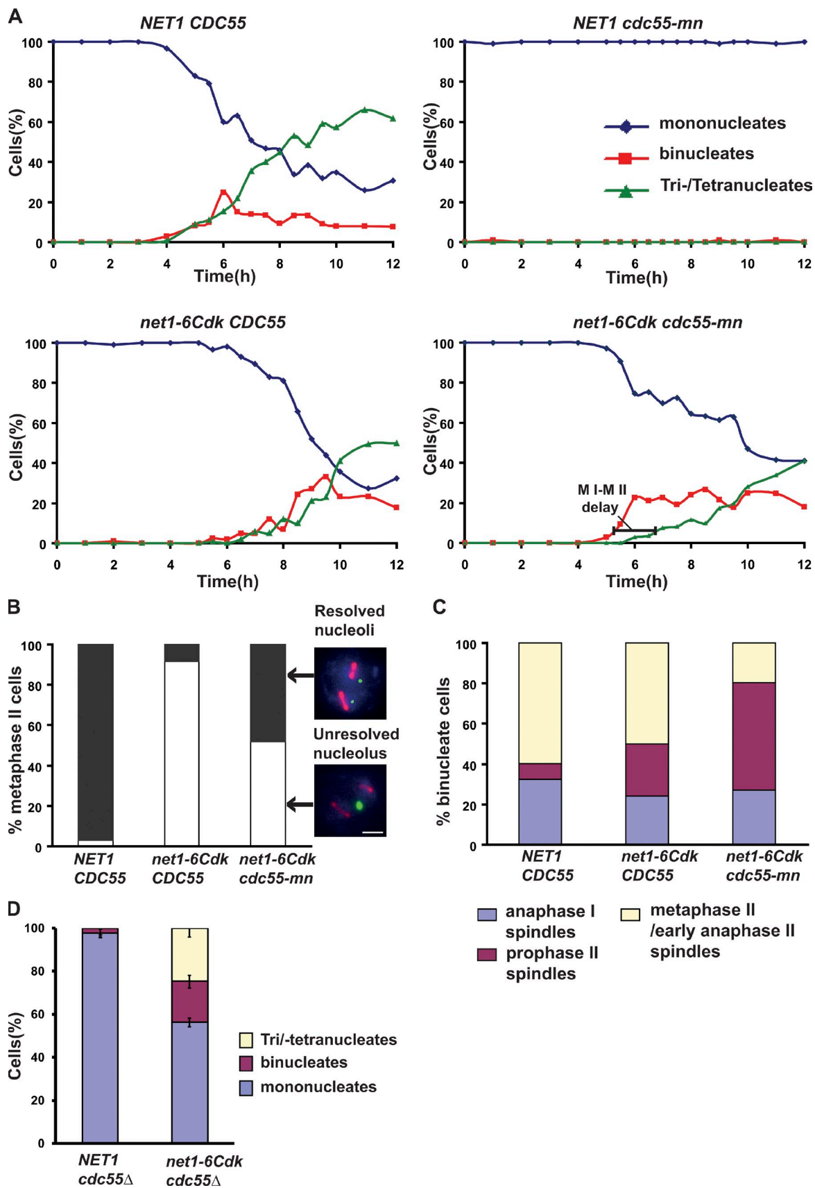
Figure 4. net1-6Cdk suppresses the nuclear division defect of cdc55-mn and cdc55Δ cells. (A) NET1 CDC55 (Y2072), NET1 cdc55-mn (Y2075), net1-6Cdk CDC55 (Y2078), and net1-6Cdk cdc55-mn (Y2081) cells were induced to sporulate. Kinetics of nuclear division was measured in the four sporulating cultures by staining cells with DAPI ( n = 200 ). Lag in the appearance of tetranucleates relative to binucleates in net1-6Cdk cdc55-mn cells is
