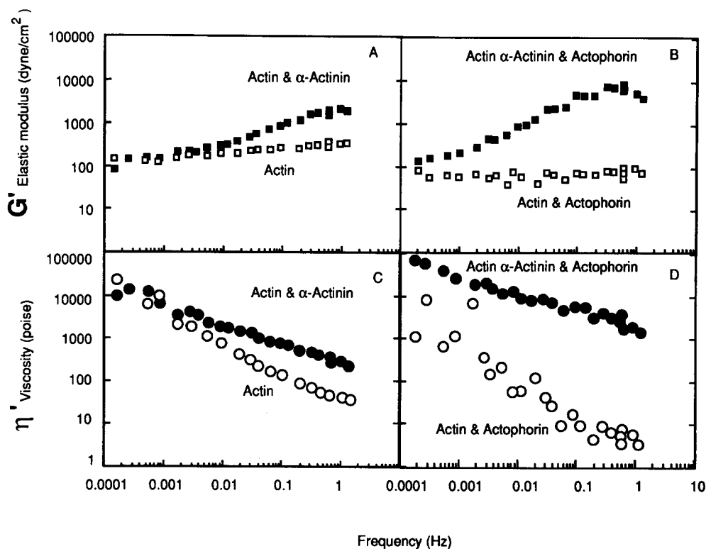
Figure 3. Quantitative rheometric measurement of the dynamic viscosity ( \circ , \bullet ) and elastic modulus ( \square , \blacksquare ), as a function of the deformation frequency. The proteins were mixed and polymerization was initiated by the addition of salts to 50 mM KCl, 1 mM MgCl 2 , 1 mM EGTA. (A) 10 \mu M actin ( \square ), or 10 \mu M actin and 2 \mu M \alpha -actinin ( \blacksquare ). (B) 10 \mu M actin and 5 \mu M actophorin ( \square ), or 10 \mu M actin, 2 \mu M \alpha -actinin, 5 \mu M actophorin ( \blacksquare ). (C) 10 \mu M actin ( \circ ), or 10 \mu M actin and 2 \mu M \alpha -actinin ( \bullet ). (D) 10 \mu M actin and 5 \mu M actophorin ( \circ ), or 10 \mu M actin, 2 \mu M \alpha -actinin, 5 \mu M actophorin ( \bullet ). The slopes of the viscosity curves by linear least squares fit to all the data are: actin, -0.74 ; actin and \alpha -actinin, -0.46 ; actin and actophorin, -0.81 ; actin, actophorin, and \alpha -actinin, -0.39 .
