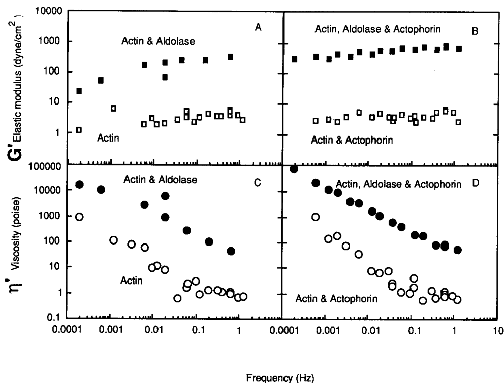
Figure 4. Quantitative rheometric measurement of the dynamic viscosity ( \circ , \bullet ) and elastic modulus ( \square , \blacksquare ), as a function of the deformation frequency. The proteins were mixed and polymerization was initiated by the addition of salt to 1 mM MgCl 2 and 1 mM EGTA. (A) 10 \mu M actin ( \square ), or 10 \mu M actin and 5 \mu M aldolase ( \blacksquare ). (B) 10 \mu M actin and 0.5 \mu M actophorin ( \square ), or 10 \mu M actin, 5 \mu M aldolase, and 0.5 \mu M actophorin ( \blacksquare ). (C) 10 \mu M actin ( \circ ), or 10 \mu M actin and 5 \mu M aldolase ( \bullet ). (D) 10 \mu M actin and 0.5 \mu M actophorin ( \circ ), or 10 \mu M actin, 5 \mu M aldolase, and 0.5 \mu M actophorin ( \bullet ). The slopes of the viscosity curves by linear least squares fit to all the data are: actin, -0.83 ; actin and aldolase, -0.76 ; actin and actophorin, -0.88 ; actin, actophorin, and aldolase, -0.80 .
