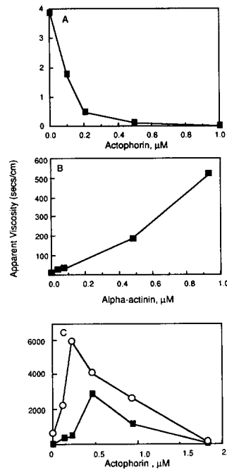
Figure 1. Falling ball viscometry of rabbit muscle actin gels polymerized in the presence of \alpha -actinin and actophorin. Polymerization was initiated by the addition of salts to 50 mM KCl, 1 mM \text{MgCl}_2 , 1 mM EGTA at 25°C. (A) 10 \mu\text{M} actin and various amounts of actophorin. (B) 10 \mu\text{M} actin and various amounts of \alpha -actinin. (C) 5 \mu\text{M} actin various amounts of actophorin and \alpha -actinin at 0.47 \mu\text{M} (■) and 0.94 \mu\text{M} (○).
