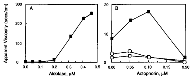
Figure 2. Falling ball viscometry of rabbit muscle actin gels polymerized in the presence of rabbit muscle aldolase and actophorin. Polymerization was initiated by the addition of salts to 1 mM \text{MgCl}_2 , 1 mM EGTA at 25°C. (A) 5 \mu\text{M} actin various amounts of aldolase. (B) 5 \mu\text{M} actin various amounts of actophorin and aldolase at 0.2 \mu\text{M} (■), 0.1 \mu\text{M} (○) and 0.05 \mu\text{M} (□).
