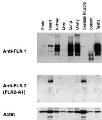
Figure 2. Western blot analysis of FLN1 and FLN2. Approximately 30 \mu g of total protein lysate from several tissues were separated by electrophoresis on a 4–20% gradient gel and transferred to nitrocellulose membranes. Anti-FLN1 and anti-FLN2 (FLN2-A1) antibodies were used to detect each protein in the tissue lysates. For FLN1, a prominent band at \sim 280 kD with several smaller bands were detected
