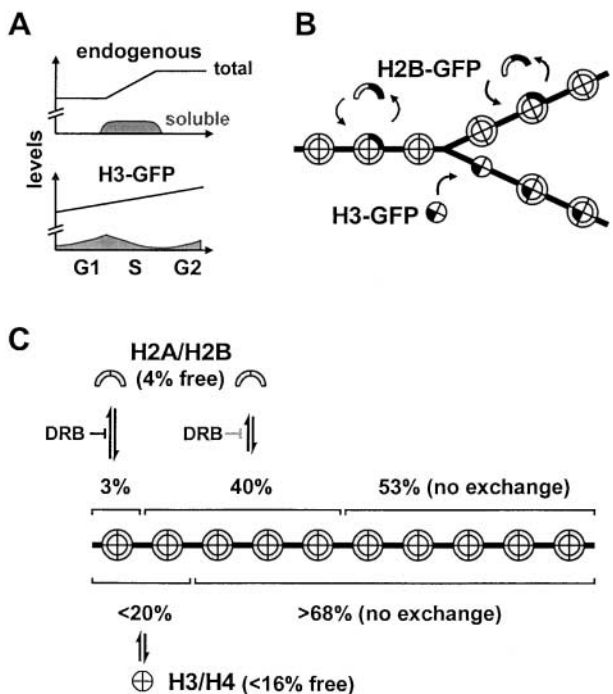
Figure 7. Models for histone exchange. (A) Changes in histone levels during the cell cycle. Endogenous histones are made mainly during S phase when a soluble pool is seen. Tagged histones are made continuously; the soluble pool that accumulates by the end of G1 phase is depleted in S phase (as histones are incorporated) and then replenished in G2 phase. (B) Incorporation of tagged histones (black areas) into chromatin. Nucleosomes are represented as circles with eight sectors, DNA as a forked line. H2B-GFP exchanges with H2B before, during (not shown), and after replication. H3-GFP is mainly incorporated into nucleosome cores near the replication fork; subsequently, it does not exchange. (C) Different kinetic populations. H2B is found in four populations: 4% diffuses freely, 3% in active transcription units exchanges rapidly ( t_{1/2} \sim 6 min), 40% in the surrounding domains exchanges slowly ( t_{1/2} \sim 130 min), and 53% in heterochromatin is essentially immobile ( t_{1/2} > 510 min). Although H2A was not studied, it is assumed to behave like H2B. H3 is found in three populations: <16% diffuses freely, <16% in and around active transcription units exchanges slowly ( t_{1/2} \sim 130 min), and >68% is essentially immobile (this constitutes >80% of the incorporated fraction). H4 behaved similarly to H3. The diffusing and slowly exchanging fractions of H3-GFP and H4-GFP are overestimated because expression of the tagged histones is unregulated. DRB affects exchange as indicated.
