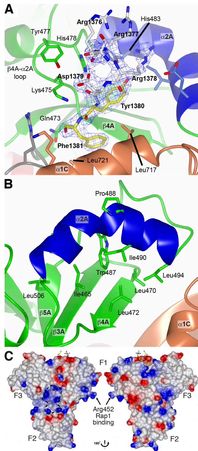
Figure 3. Structural details of the HEG1 binding pocket in KRIT1. (A) Electron density of the HEG1 peptide in complex with the KRIT1 FERM domain. Electron density [ 2F_o - F_c map contoured at 1.2\sigma ] of the HEG1 peptide. The HEG1 peptide is colored as in Fig. 2 C, and the KRIT1 FERM domain is as in Fig. 2 B. Some of the key KRIT1 residues are highlighted. (B) Close view of the novel helix \alpha 2A in the KRIT1 F1 domain. The helix is kinked by \sim 70^\circ in the middle because of the presence of Pro 488 . The helix position is stabilized by hydrophobic contacts with residues from the \beta sheet. (C) The surface charge map of the KRIT1 FERM domain shows a basic surface at the F1–F2–F3 subdomain interface. The position of Arg452 is highlighted as mutation of this residue to Glu reduces KRIT1 binding to Rap1.
