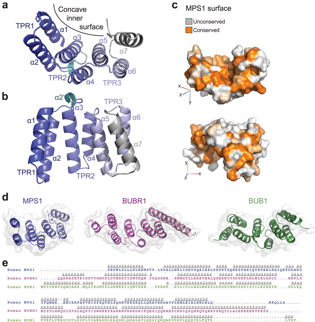
Figure 1. Crystal structure of the MPS1 TPR domain. (a) Crystal structure of the TPR domain. A cartoon diagram of the three TPR1–3 helical doublets forming the concave surface is shown in blue shades that fade toward gray from the N toward the C terminus; the C-terminal helix is in gray, and the \alpha 2' short helix between TPR1 and TPR2 is in cyan. (b) A side view of the TPR domain. (c) A surface representation of the TPR domain colored by sequence conservation among vertebrate MPS1 TPR domains; the top view emphasizes the conservation of the concave inner surface, and the bottom view shows some conserved patches on the generally unconserved outer surface. (d) The TPR domains of MPS1, BUBR1, and BUB1 are shown in the same orientation after structural superposition, as cartoon diagrams within a transparent surface. (e) The sequence alignment resulting from the structural superposition of the three TPR domains above is shown together with secondary structure elements. Dots indicate gaps. Loops indicate helices.
