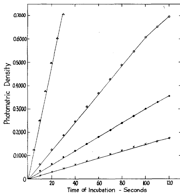
FIG. 1. Formation of red pigment by 0.25 (x), 0.5 (•), 1.0 (◊), and 4.0 (Δ) μg. of a commercial peroxidase preparation. Incubation at 20°C.; pH 6.25.
