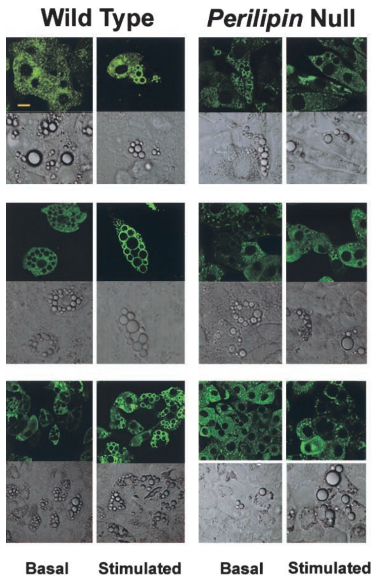
Figure 3. HSL fails to translocate in adipocytes differentiated from perilipin -null embryonic fibroblasts on stimulation. Embryonic fibroblasts from wt and perilipin -null mice were differentiated into adipocytes as described under Materials and methods. Basal cells were incubated with 100 nM PIA and stimulated cells for 10 min with 10 \mu M isoproterenol. After 10 min of stimulation, cells were fixed and immunostained with affinity-purified rabbit anti-HSL antibodies and FITC-conjugated goat anti-rabbit antibodies. Bar, 10 \mu m. Top, middle, and bottom rows show representative cells from three of four rounds of differentiation performed using fibroblasts derived from four different embryos of each phenotype.
