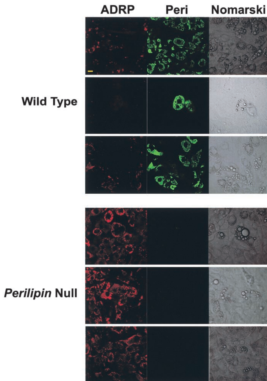
Figure 2. ADRP replaces perilipin on lipid droplets in embryonic fibroblasts derived from perilipin -null mice.
