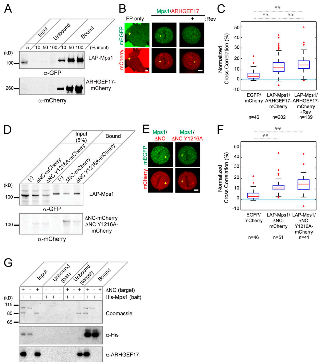
Figure 4. ARHGEF17 and Mps1 interact during mitosis. (A) Coimmunoprecipitation of ARHGEF17 with Mps1: LAP-tagged Mps1 (LAP-Mps1) and mCherry-tagged ARHGEF17 (ARHGEF17-mCherry) were immunoprecipitated using GFP-binding protein coupled to agarose beads. Input, supernatants (Unbound), and immunoprecipitates (Bound) were analyzed by Western Blot (anti-GFP and anti-mCherry). (B and C) FCCS of Mps1 and ARHGEF17. Exemplary cells (B; yellow crosses mark position for FCCS measurement) and normalized cross-correlation (C) of ARHGEF17-mCherry and LAP-Mps1 with or without reversingine treatment of >40 cells (specific numbers indicated)/three independent experiments. (D) Coimmunoprecipitation of ARHGEF17 fragments with Mps1: LAP-Mps1 and mCherry-tagged ARHGEF17 fragments ( \Delta NC-mCherry and \Delta NC Y1216A-mCherry) were precipitated using GFP-binding protein coupled to agarose beads. Input and precipitates were analyzed by Western blot (anti-GFP and anti-mCherry). (E and F) FCCS of Mps1 and ARHGEF17 fragments. Exemplary cells (E) and normalized cross-correlation (F) of LAP-Mps1 and ARHGEF17 fragments ( \Delta NC-mCherry and \Delta NC Y1216A-mCherry) of >40 cells (specific numbers indicated)/three independent experiments. (G) In vitro pull-down of ARHGEF17 fragments with Mps1. His-tagged Mps1 (bait) and untagged ARHGEF17 fragments ( \Delta NC; target) were precipitated using His-tag binding protein coupled to Talon beads. Input, supernatants (Unbound), and precipitates (Bound) were analyzed by Western blot (anti-His-tag [middle] and anti-ARHGEF17 [bottom]). Coomassie brilliant blue staining was used as internal protein control in each condition. Boxes show median, 25–75%; whiskers show 1.5 \times interquartile range. **, P < 0.01 by two-tailed unpaired Student's t test, compared with mEGFP and mCherry (C and F) or between metaphase and metaphase with reversingine treatment (F). Slower migration of Mps1/ARHGEF17 bands could be caused by phosphorylation (A and D). Bars, 5 \mu m.
