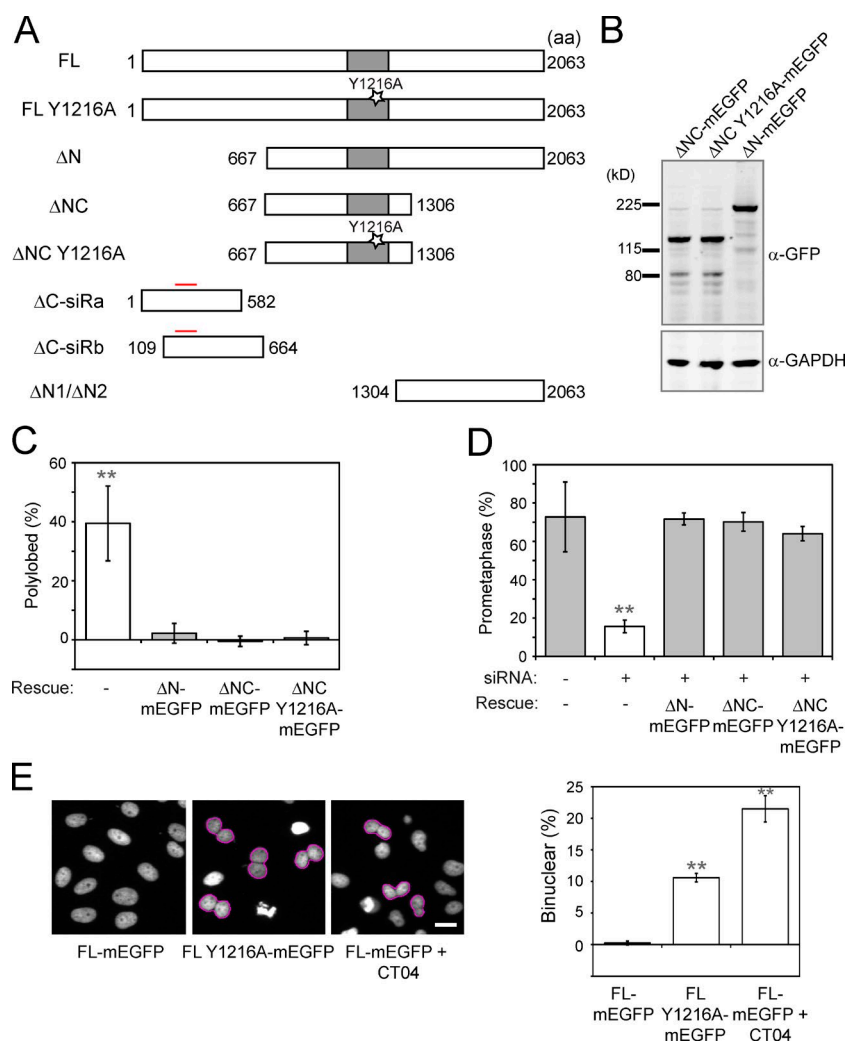
Figure 2. ARHGEF17 fragment restores SAC function independently of catalytic activity for Rho GEF of ARHGEF17. (A) Schematic depiction of hARHGEF17 variants used in phenotypic rescue assays: FL: hARHGEF17 (1–2,063)-mEGFP; FL Y1216A: hARHGEF17 (1–2,063)-Y1216A-mEGFP; ΔN: hARHGEF17 (667–2,063)-mEGFP; ΔNC: hARHGEF17 (667–1,306)-mEGFP; ΔNC Y1216A: hARHGEF17 (667–1,306)-Y1216A-mEGFP; ΔC-siRa: hARHGEF17 (1–582)-mEGFP; ΔC-siRb: hARHGEF17 (109–664)-mEGFP; ΔN1: mEGFP-hARHGEF17 (1,304–2,063)-mEGFP; and ΔN2: hARHGEF17 (1,304–2,063)-mEGFP. Gray boxes indicate GEF activity domain (Dbl-homologous domain); Y1216A indicates the inactivating mutation in the GEF domain; red lines indicate sites for mutations for siRNA resistance. (B) Immunoblot analysis of hARHGEF17 fragments fused to GFP (detected with anti-GFP). GAPDH, loading control. (C and D) Rescue of hARHGEF17 knockdown-induced polylobulation (C) or SAC defect (D). Comparison of polylobed (C; normalized to Scrambled) or prometaphase population (D; nocodazole treated) rescued with hARHGEF17 fragments (ΔN-mEGFP, ΔNC-mEGFP, and ΔNC Y1216A-mEGFP) of >11,500 (C) or >6,300 (D) cells/three independent experiments. (E) Phenotypic analysis of cytokinesis defects (binuclearity) of a catalytically inactive mutant of full-length ARHGEF17 (FL Y1216A) during mitosis. (left) H2B-mCherry, wild-type full-length (FL-mEGFP), catalytically inactive (FL Y1216A-mEGFP), or cells 24 h after CT04 treatment (0.25 mg/ml; FL + CT04). (right) Comparison of binuclear population of >3,000 cells/three independent experiments. Bar graphs show mean ± SD. **, P < 0.01 by two-tailed unpaired Student's t test, compared with no rescue construct (C), si(Scrambled) without a rescue construct (D), or FL-mEGFP (E). Cells automatically segmented/analyzed by CellCognition. Bars, 10 μm.
